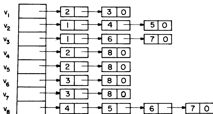
Figure 6.13 Graph G and Its Adjacency Lists.
