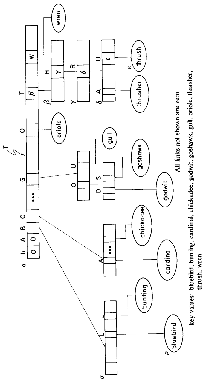
Figure 10.18 Trie created using characters of key value left to right, one at a time
