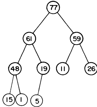
Initial Heap
