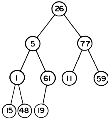
Input File
